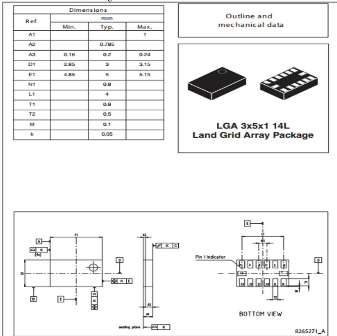
Figure 20 – LSM303DLHC Dimensions
